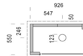
Location of the replacement air pipe Deko 7R Uno
